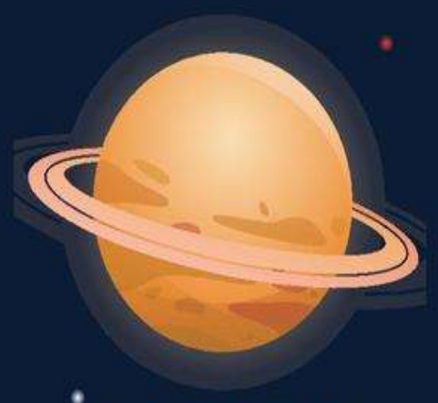
SATURN
